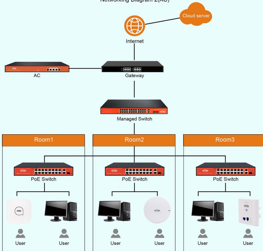
Networking Diagram 2(AC)
